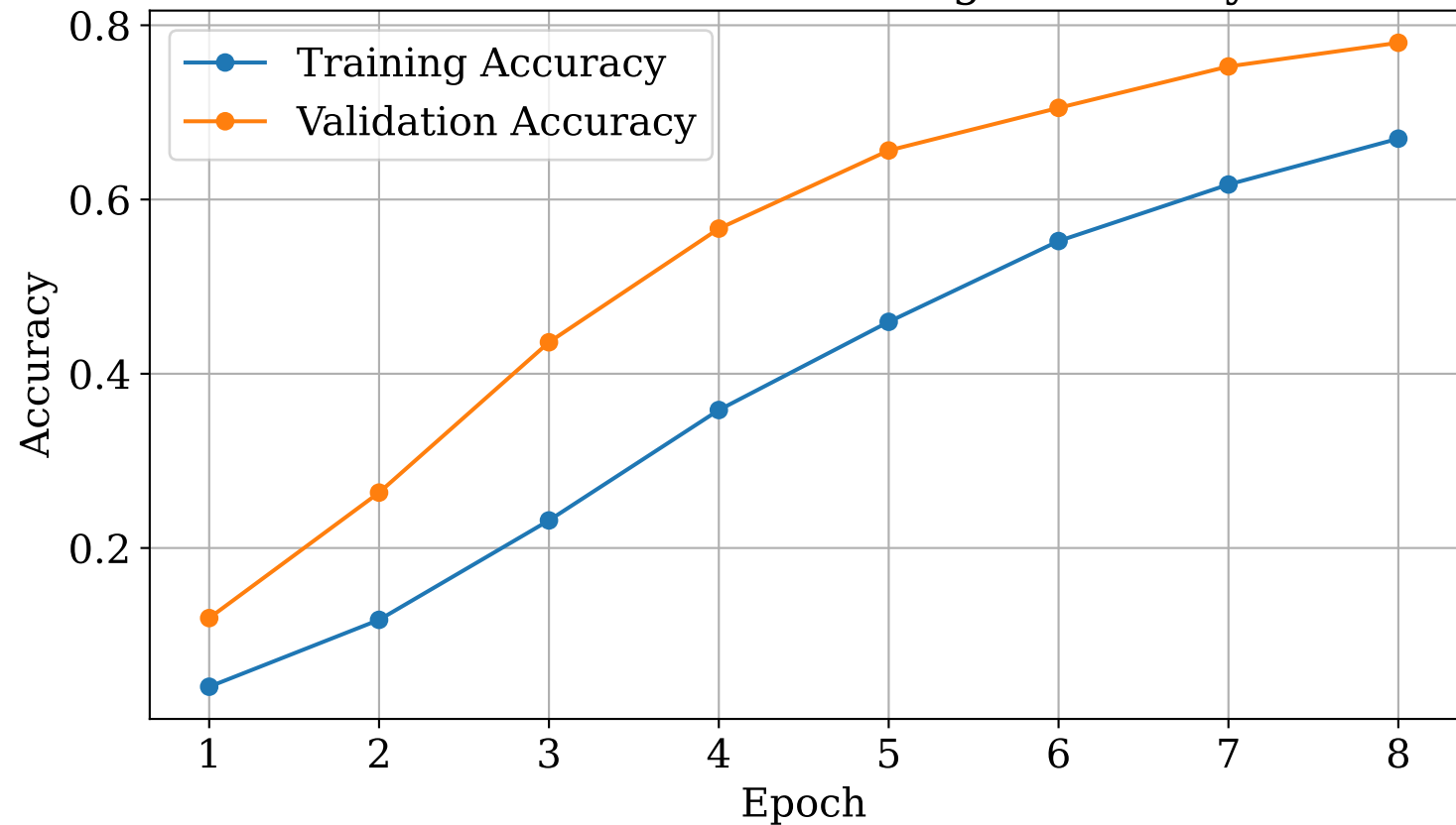
MobileNetV2 Fine-Tuning - Accuracy
